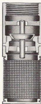
Foot Valve With Strainer Poppet Type
