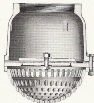
Foot Valve With Strainer Hinged Type
