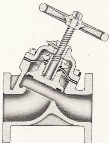
Y-Pattern Globe Valve With Stem 60 degrees from Run
