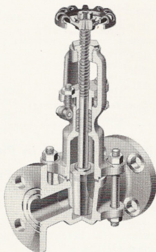
Plug Gate Valve
