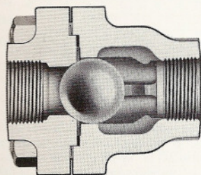
In-Line Ball Check Valve
