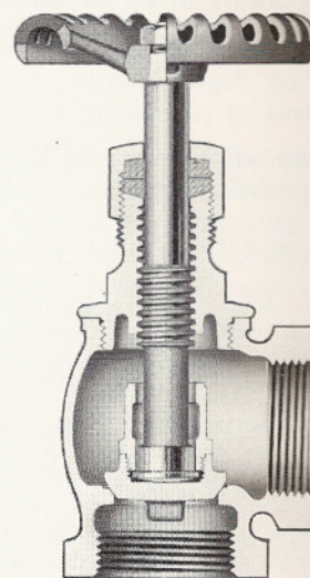
Conventional Angle Valve
