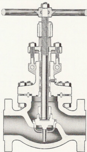
Conventional Globe Valve With Disc Guide
