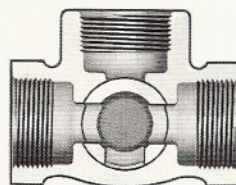
Three-Way Cock Sectional and Outside Views
